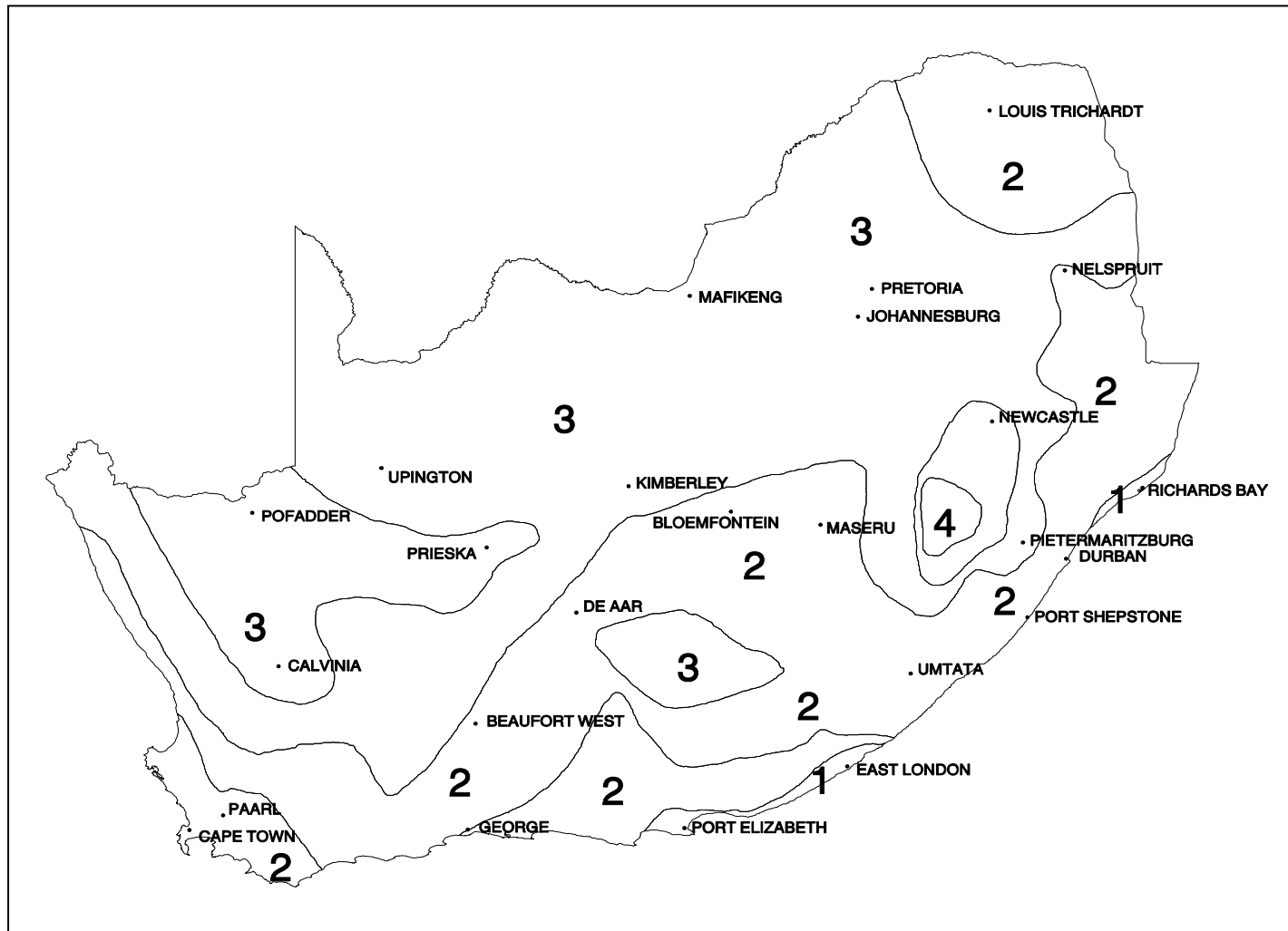
Figure 5.3 Design rainfall intensity distribution types over southern Africa (after Weddepohl, 1988)
