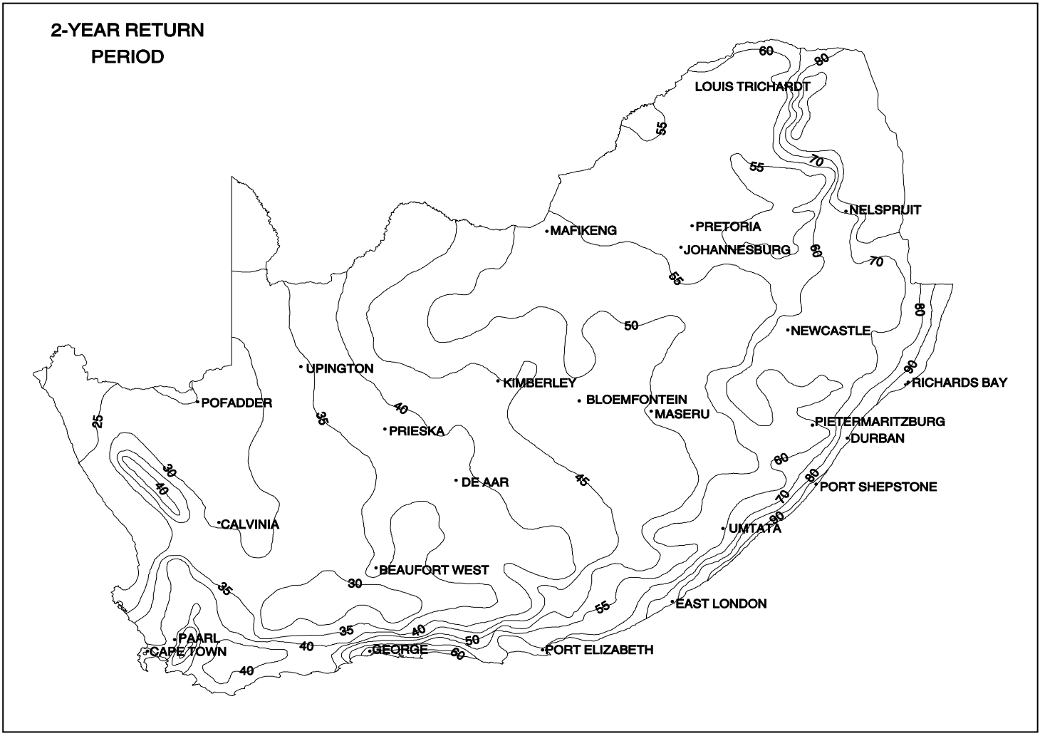
Figure 5.2 One-day design rainfall distribution over southern Africa for selected return periods (after Schmidt and Schulze, 1987a)
